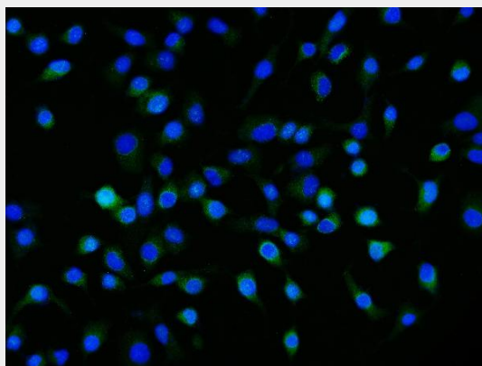
Figure 2. IF analysis of Neuropilin 1 using anti-Neuropilin 1 antibody (M01324-2). Neuropilin 1 was detected in an immunocytochemical section of A549 cells. Enzyme antigen retrieval was performed using IHC enzyme antigen retrieval reagent (AR0022) for 15 mins. The
