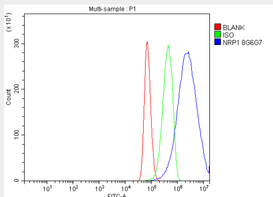
Figure 3. Flow Cytometry analysis of U737 cells using anti-Neuropilin 1 antibody (M01324-2). Overlay histogram showing U737 cells stained with M01324-2 (Blue line). The cells were blocked with 10% normal goat serum. And then incubated with mouse anti-Neuropilin 1 Antibody (M01324-2, 1 \mu\text{g}/1 \times 10^6 cells) for 30 min at 20°C. DyLight®488 conjugated goat anti-mouse IgG (BA1126, 5-10 \mu\text{g}/1 \times 10^6 cells) was used as secondary antibody for 30 minutes at 20°C. Isotype control antibody (Green line) was mouse IgG (1 \mu\text{g}/1 \times 10^6 ) used under the same conditions. Unlabelled sample (Red line) was also used as a control.
